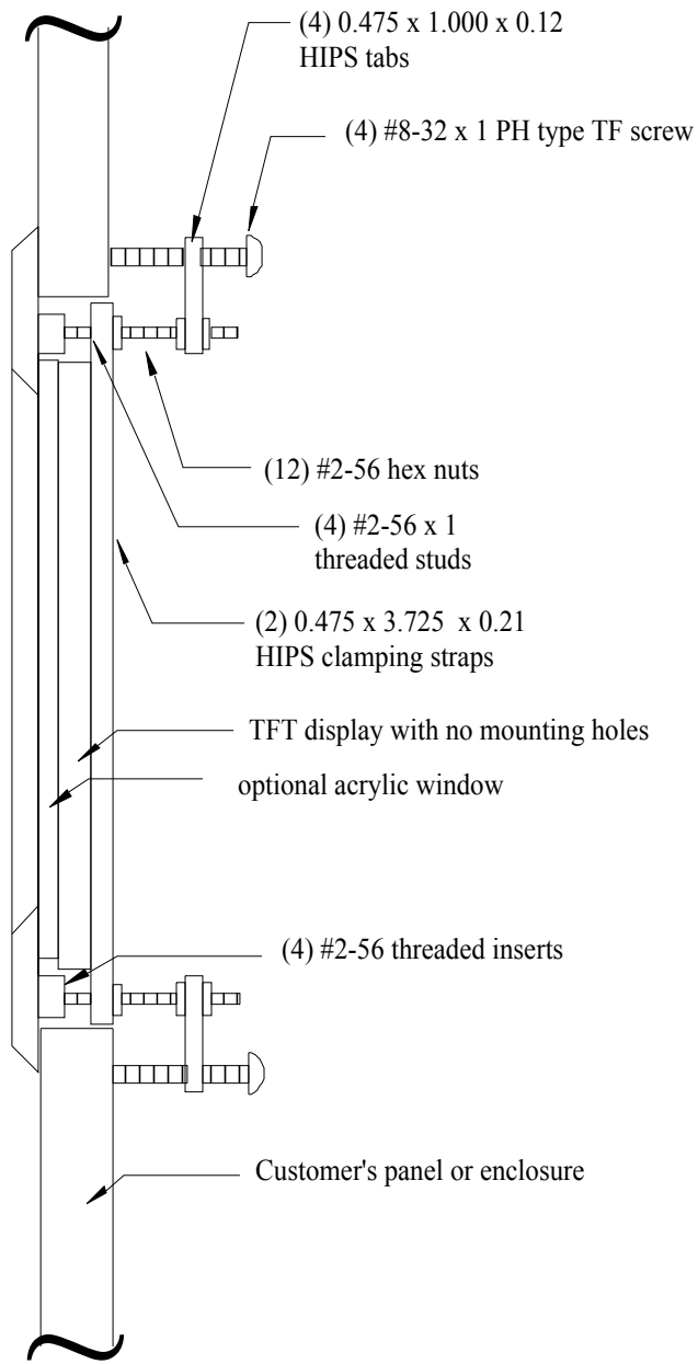
Typical TFT Bezel Mounting 5.7" & 7.0" use #4-40 threaded studs, nuts
