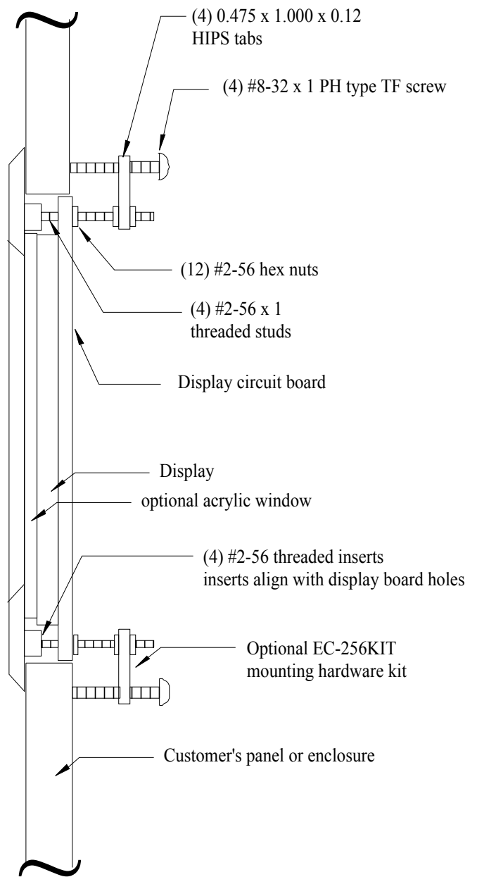
Typical Display Bezel Mounting (displays with mounting holes)
